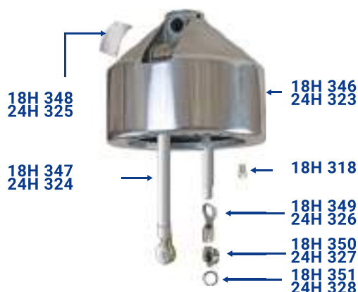
18H MACKHAUL / SUPERHAUL GILL SPINNING FRAME 24H DOUBLE ROW GILL SPINNING FRAME
